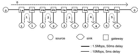
Figure 1: Simulation network with 5 congested gateways.
