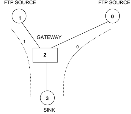
Figure 13: Simulation network with one congested gateway.
